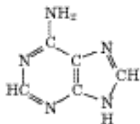
Adenine
